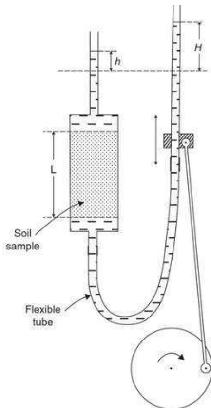
Figuur 2-45: Oscillating permeameter (bron: Cooper, 2016)
